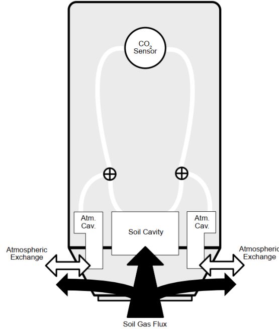
Figure 1: Internal view of the eosFD chamber, depicting the exchange of atmospheric gases and soil (sample) flux with the chamber cavities. Source: nickerson2018<empty citation>.
